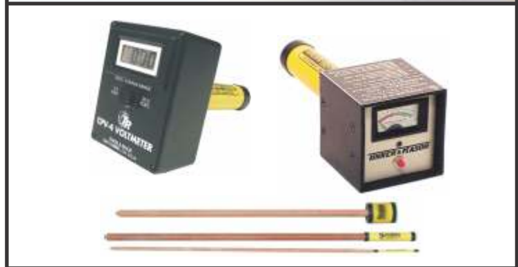
Half Cells, CP Voltmeters and Extension Handles
